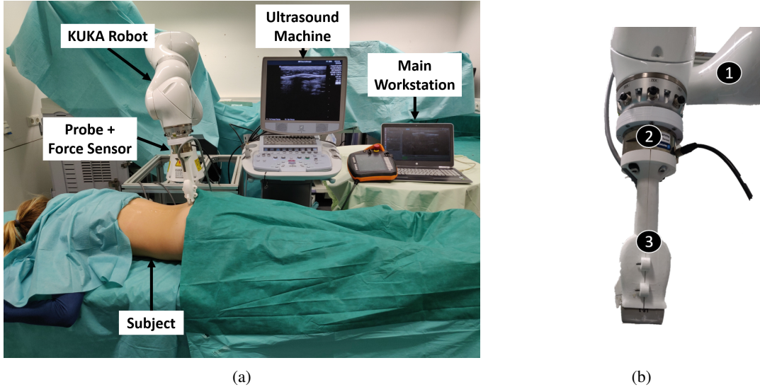
Fig. 1: a) The Robotic Ultrasound System for Vertebral Level Classification Setup. b) The Robot end-effector configuration: 1 - Robotic arm, 2 - External force sensor, 3 - Ultrasound linear probe + 3D printed probe holder.
