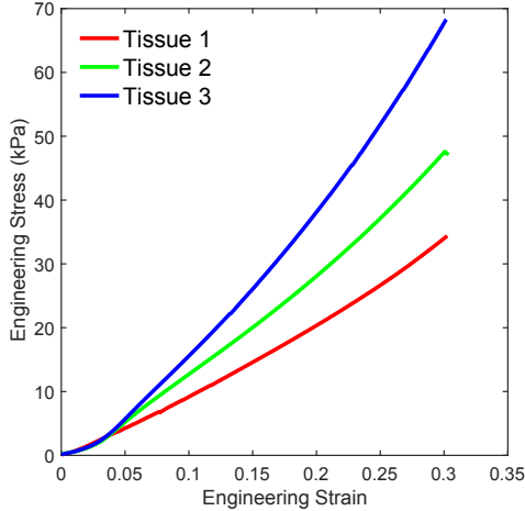
Fig. 6. Stress vs. strain curve of SEBS soft tissue simulants. The Young's modulus of each tissue is obtained by finding the slope of the linear section of the curves. Tissue 1, 2, and 3 are 15%, 20%, and 25% G1650 SEBS in mineral oil soft tissue simulants, respectively.
