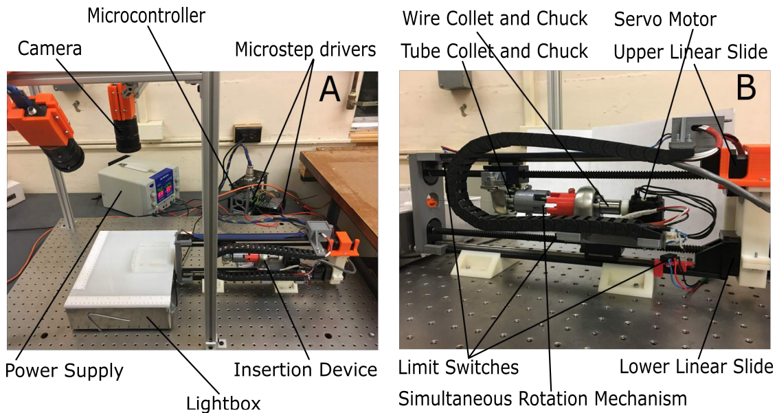
Fig. 5. (A) The whole needle insertion system setup including the insertion device, two micro step drives that drive linear slides, a lightbox, a camera, a microcontroller, and a power supply. (B) Insertion device setup, including three limit switches, simultaneous rotation mechanism 3D printed by ABS, tube and wire collets and chucks, two linear slides and two bearings.
