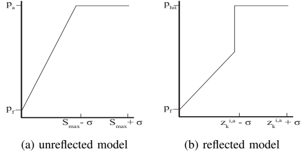
Fig. 2: Illustrative plots of the functions (a) l_u and (b) l_r . The x -axis in both plots measures s_{m_j^i}^a , the distance between the a^{\text{th}} laser range sensor of robot R^i and any grid cell m_j^i that intersects the beam from this laser, which yields the distance measurement z_k^{i,a} at time step k .
