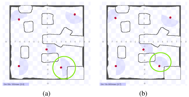
Fig. 8: The robot inside the green circle (a) detects an obstacle, then (b) follows a new heading computed from Eq. (5).
