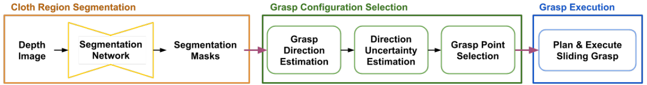
Fig. 2: Pipeline for our method. Cloth region segmentation takes a depth image and outputs segmentation masks for cloth edges and corners. Grasp selection uses the masks to compute a grasp point and direction in the camera frame. Grasp execution transforms the grasp configuration into the robot frame and executes the grasp.
