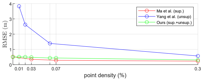
(a) RMSE comparison to [16] and [22]
