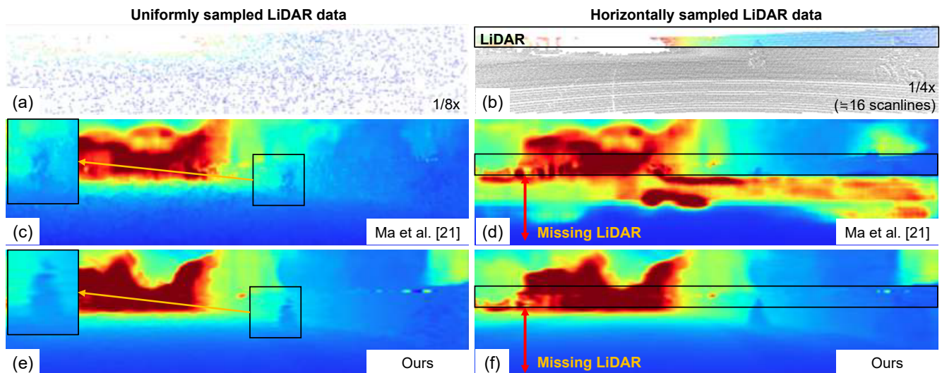
Fig. 5: Qualitative comparison to Ma et al. [21] given the sparse and bias LiDAR measurements in the KITTI dataset. (a) and (b) Uniformly sampled LiDAR data and horizontally sampled LiDAR data. The depth map from (c) and (d) result from Ma et al. [21]. And the depth maps from (e) and (f) result from the proposed method. The results show that the proposed method is more robust on the sparsity or bias change of range measurements than Ma et al. [21].
