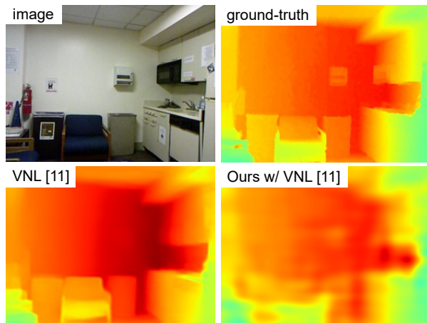
Fig. 9: Qualitative result in the NYU-Depth-V2 dataset. Our method successfully recovers an indoor depth image given 500 uniformly distributed samples (point density of 0.7%).
