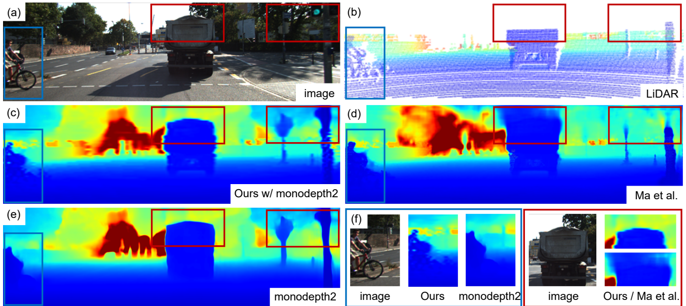
Fig. 4: Qualitative comparison to monodepth2 [9] and Ma et al. [21] over the KITTI dataset. In all sample figures, the warmer color denotes farther distance. (a) and (b) The RGB image and LiDAR raw data. Depth map from (c) the proposed method, (d) Ma et al. [21], and (e) monodepth2 [9] are shown respectively. The blue box represents our improvement from monodepth2. The red box illustrates that our method keeps the shape of a truck better than Ma et al. [21] in the region without LiDAR data.
