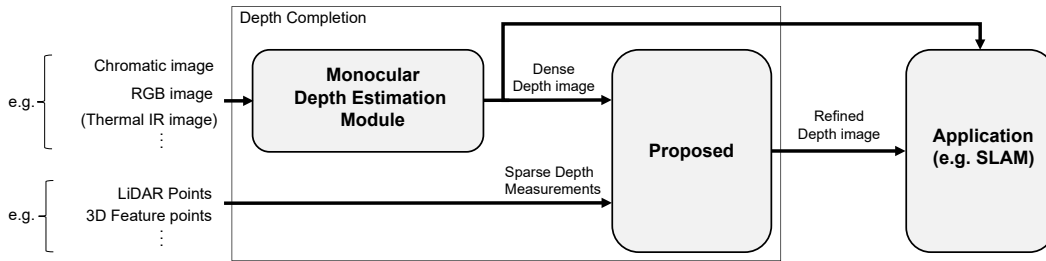
Fig. 2: System diagram. The proposed method utilizes a state-of-the-art depth prediction module specifically designed for each imaging modality. Then together with sparse depth measurements such as LiDAR, a depth regression is performed to make a refined depth image using the Gaussian process (GP).
