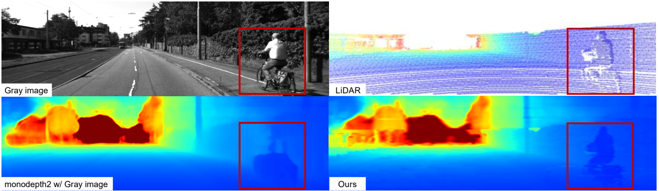
Fig. 7: Qualitative result of the proposed method that used a different imaging modality. For a given gray image on the top left, the red box represents a man riding a bicycle. The depth image is worse than its original output (bottom left) due to the different modality. The proposed method successfully recovers the shape of a man riding a bicycle (bottom right).
