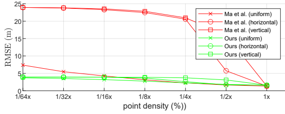
(a) RMSE comparison to [21] against LiDAR points' sparsity and bias
