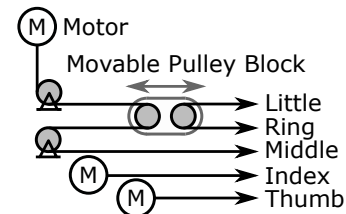
Fig. 2. Tendon-based actuation scheme of the hand: Two separate motors are used for actuation of the index finger and thumb. A third motor actuates middle, ring and little finger using an adaptive mechanism for equal force distribution.
