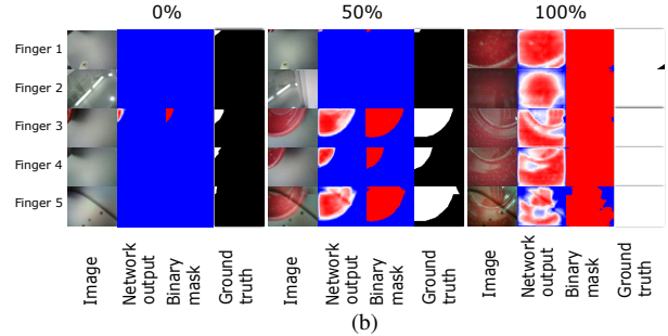
Fig. 7. a) Setup and exemplary grasped object b) Camera stream and segmentation during a grasp experiment with the bowl including the result and ground truth data. The percentage values indicate temporal progress of the grasp execution.
