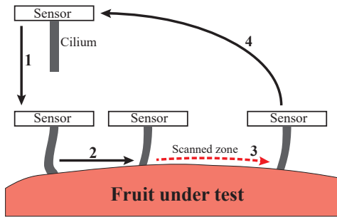
Fig. 3. Scanning sequence of the sensor. This sequence is repeated 10 times for each zone.
