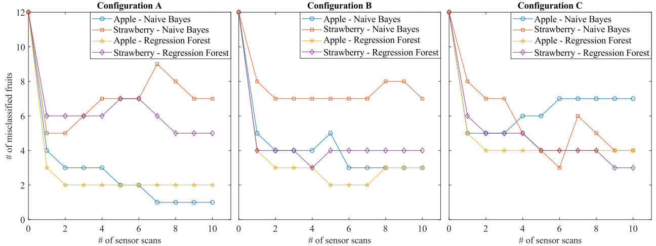
Fig. 6. Number of misclassified fruits for the three used sensor configurations as a function of the number of sensor scans over the fruit surface.
