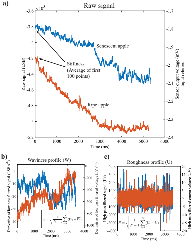
Fig. 5. Measured signal for an apple scan and derived values. a) Raw signal of the scan for a ripe and a senescent apple. b) Waviness profile, computed by low pass filtering and deriving the raw signal, used to determine the smoothness metric (inset). c) Roughness profile, computed by high pass filtering the raw signal, used to determine the texture metric (inset).
