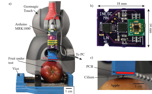
Fig. 1. a) Full experimental setup. b) Detail of the data acquisition PCB with mounted cilia. c) Single cilia scanning an apple surface. The red rectangle indicates where the data acquisition PCB is located.
